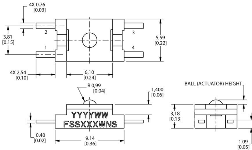
Figure 3. Packaging Dimensions (For reference only.)
