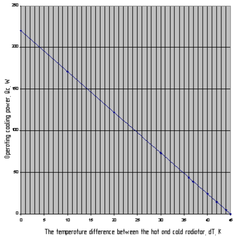
Load curve
