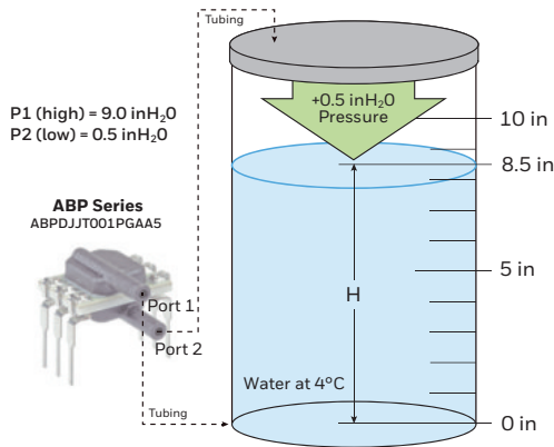
Figure 2. Pressurized Container
